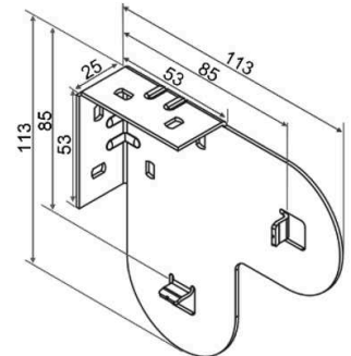
DOUBLE BRACKET
